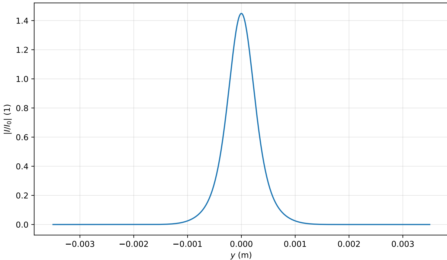
Intensity profile I(x=0, y, z=1.115)/I_0 , P_{in}=0.9P_{cr} , artificial time
